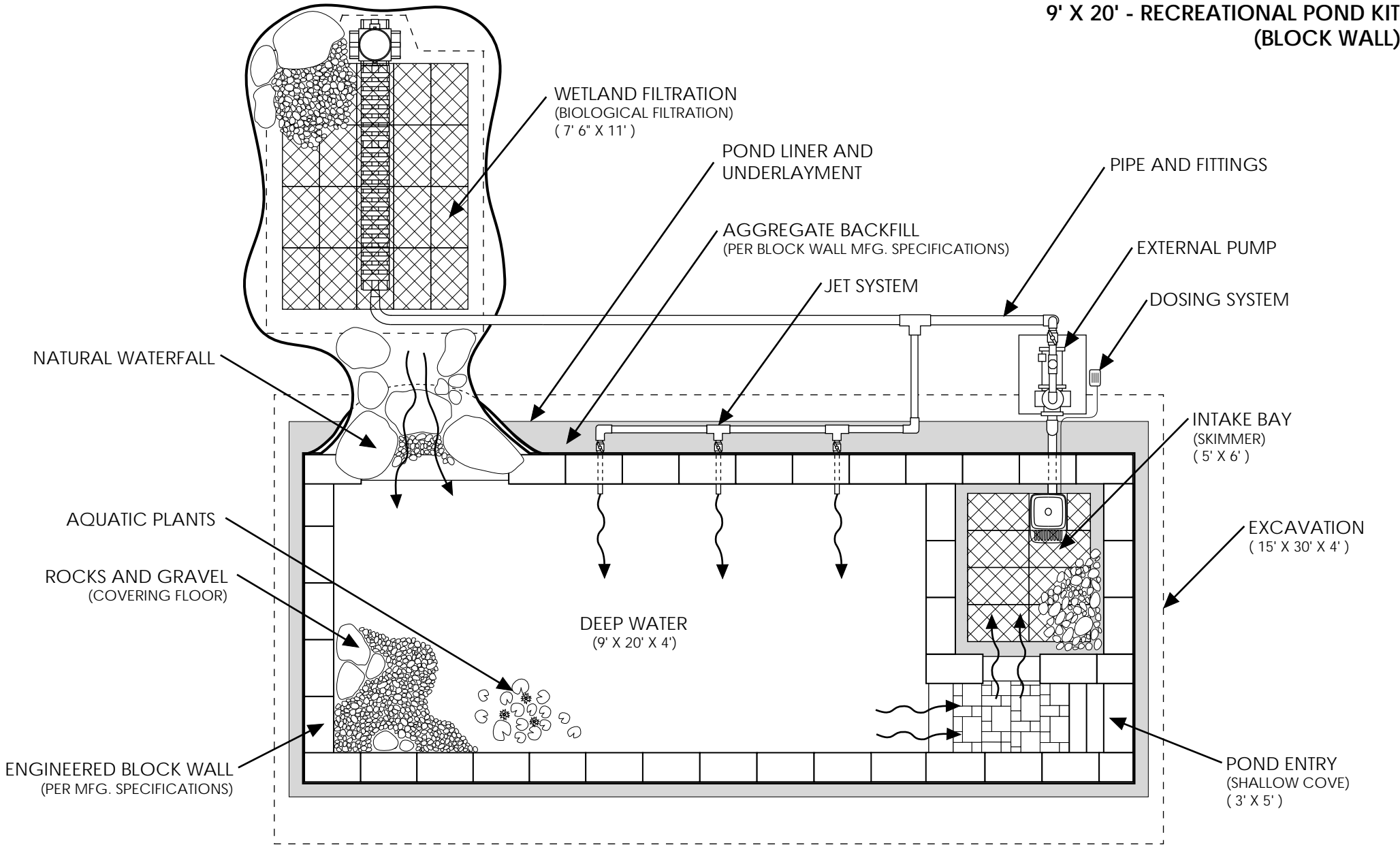
PLAN VIEW LAYOUT
