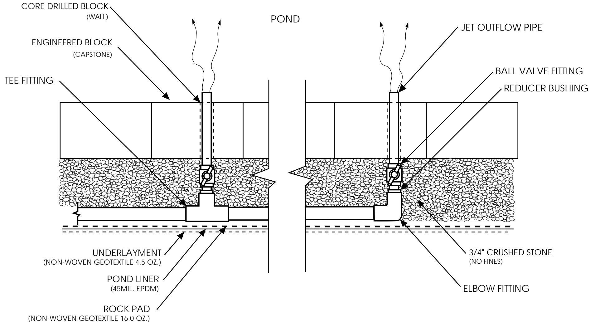
PLAN VIEW PLUMBING LAYOUT DETAIL
